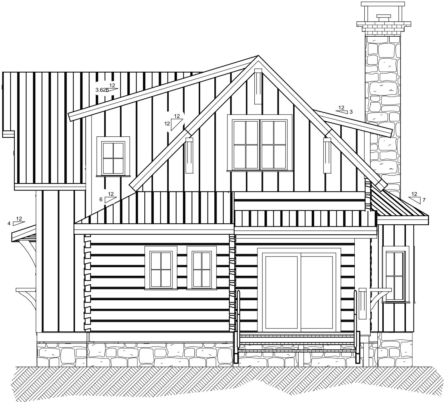
REAR ELEVATION
