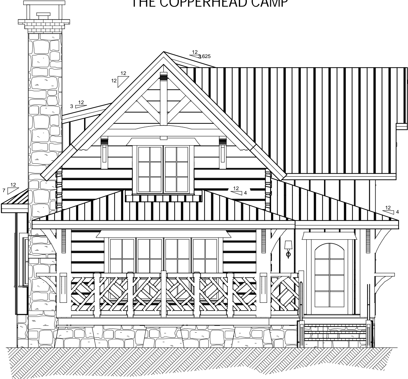
FRONT ELEVATION
